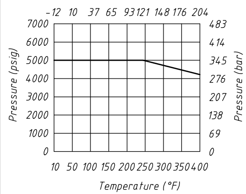
Pressure vs. Temperature Temperature ( °C)
