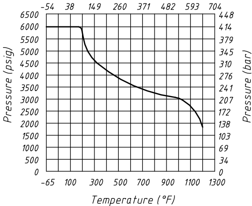
Pressure vs. Temperature Temperature ( °C)
