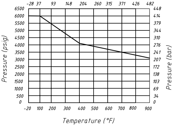
Pressure vs. Temperature Temperature (°C)
