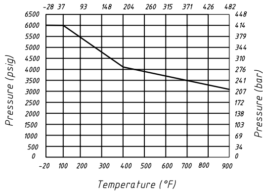
Pressure vs. Temperature Temperature (°C)
