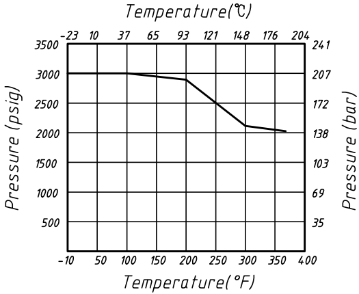
Temperature pressure curve
